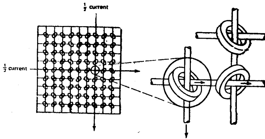
Magnetic core plane.
