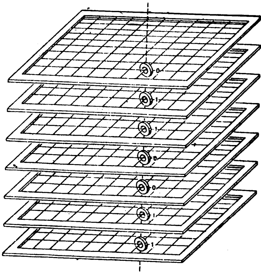
Magnetic core plane.
