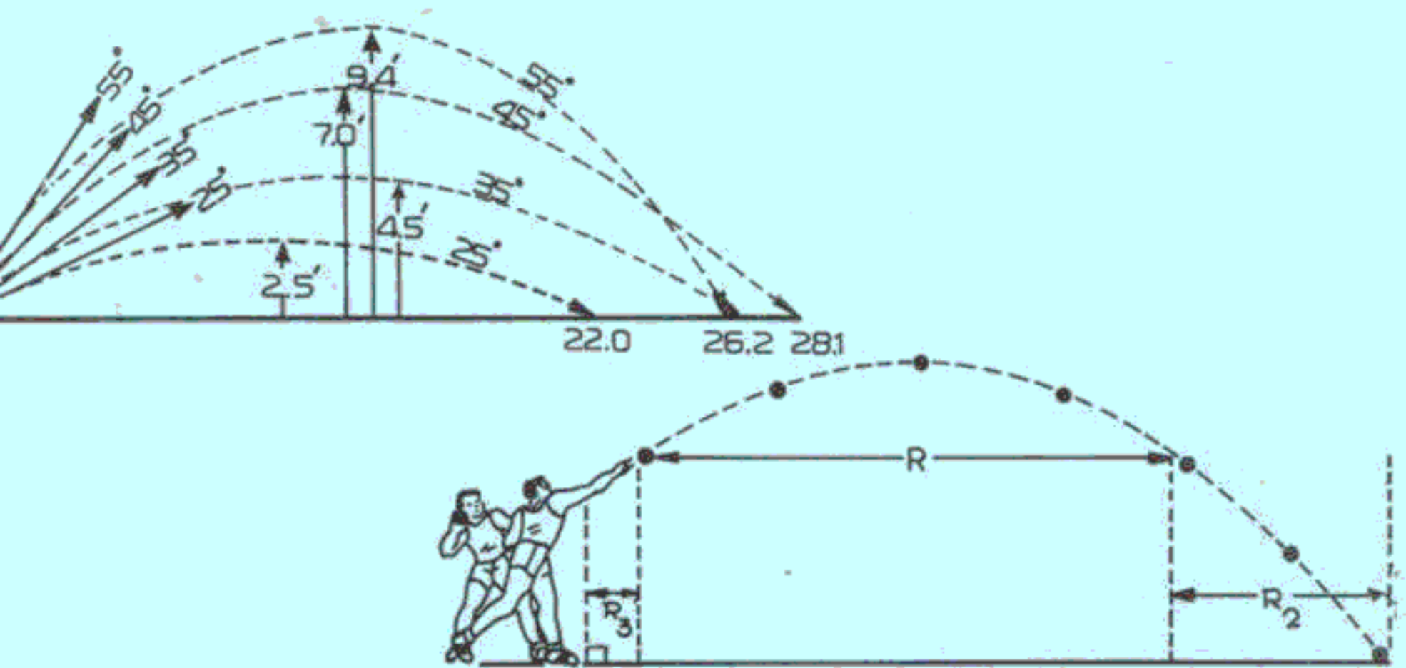
The flight of the shot. The distances R + R_2 + R_3 represent the total distance of the put.
