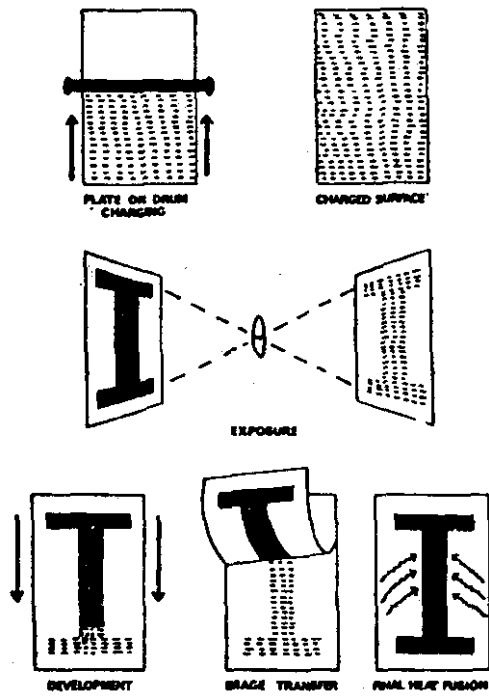
The principle of xerographic printing
