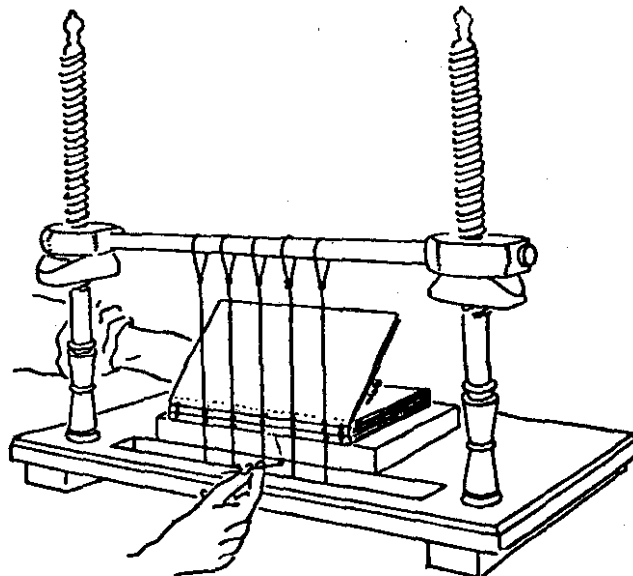
A sewing frame
