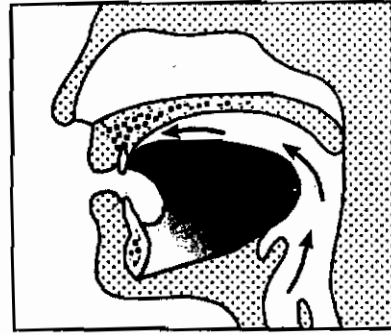
/t, d/
