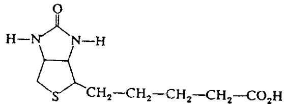
Biotin
