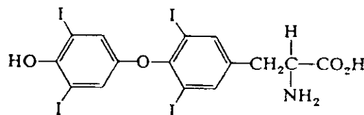
Thyroxine
